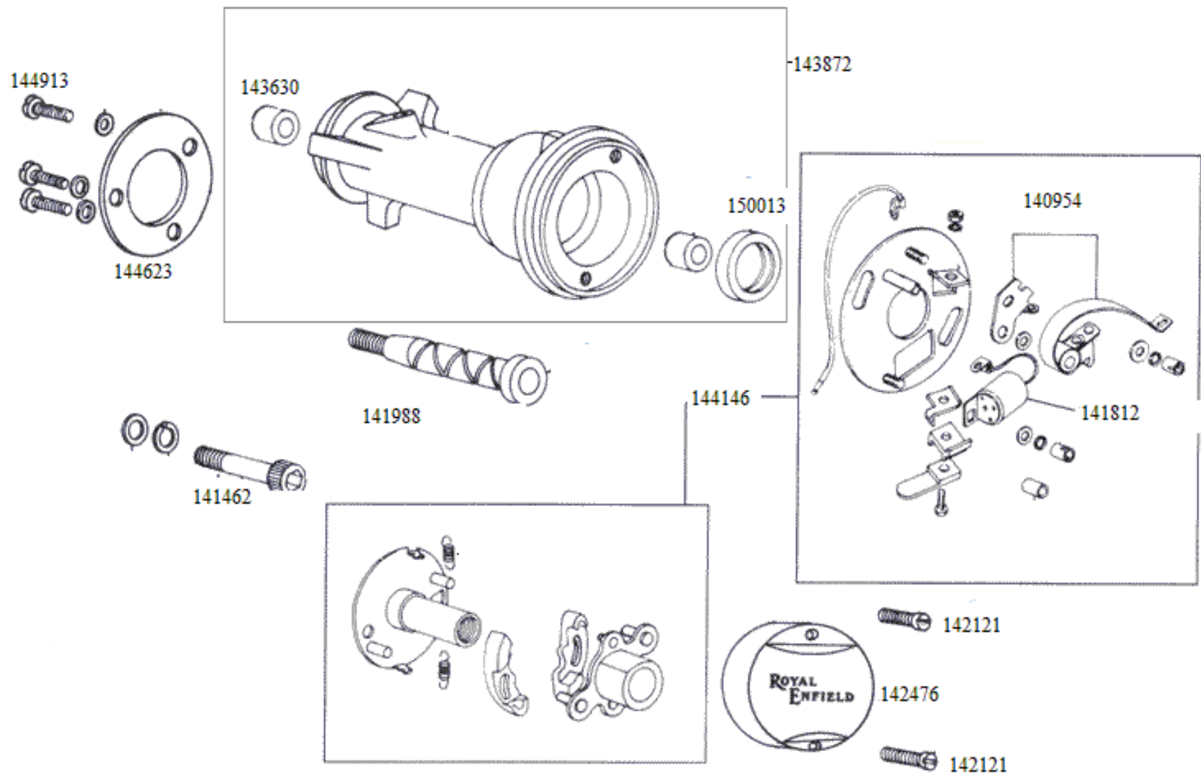
distributor 350cc
